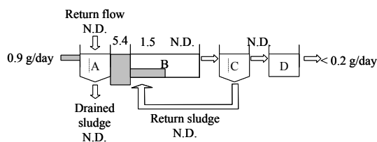
Figure 1 Mass balance of ibuprofen in WWTP
